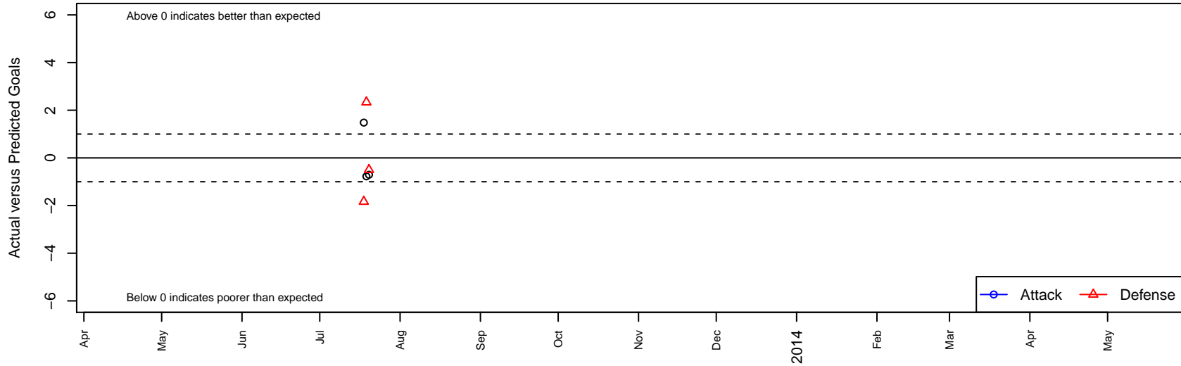
Silver Lake Adriatic B98 Dots are actual minus expected GF (blue circles) and GA (red triangles). Blue line is smoothed change in attack strength. Red is smoothed change in defense strength.
